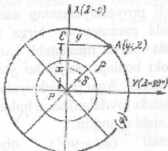
26-rasm. Normal azimutal proyeksiya koordinatalari tizimi
