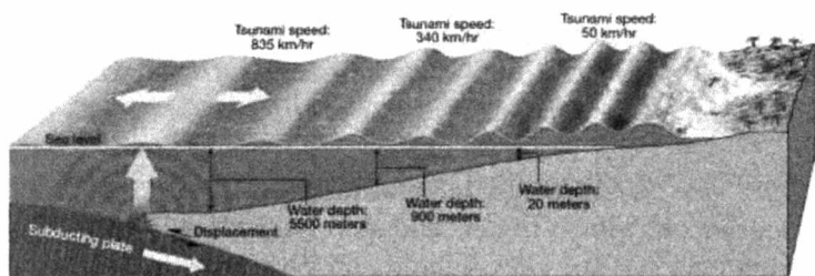
5.22-rasm. Sunamining hosil bo'lish jarayoni
