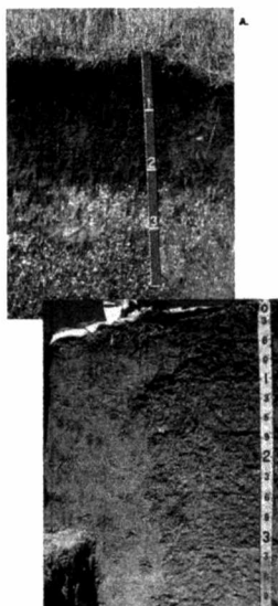
14.11-rasm. Tuproq nurashi.
