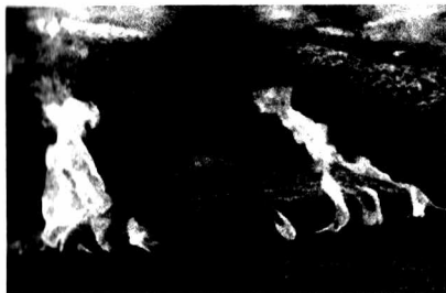
5.16-rasm. Oqayotgan lava. www.liveinfo.ucoz.com
