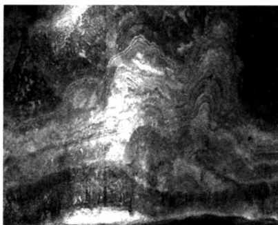
12.11-rasm. Aragonit kristallari. www/Saga.ua
