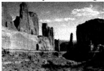
14.5 - rasm. Suv eroziyasi tufayli shakllangan dara . www.artphotoclub.com
