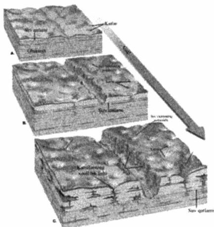
14.9-rasm. Karbonatli jinslarning karstlanishi.
