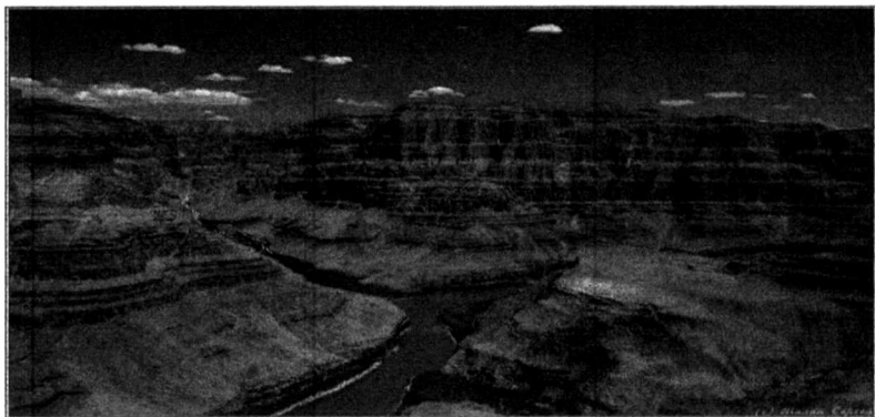
10.2 - rasm. Buyuk Kanyondagi qayirusti supalari.
