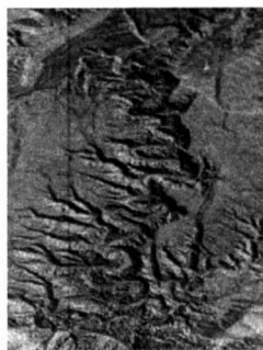
10.7-rasm. Fish-river kanyonning fazodan ko‘rinishi. www.fototerra.ru
