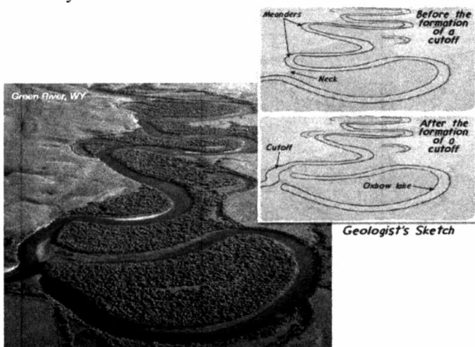
10.9-rasm. Yashil daryosining meandrlanishi.
